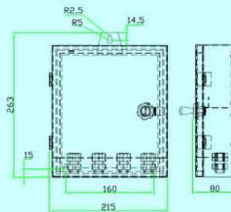
2. Shape Dimension
